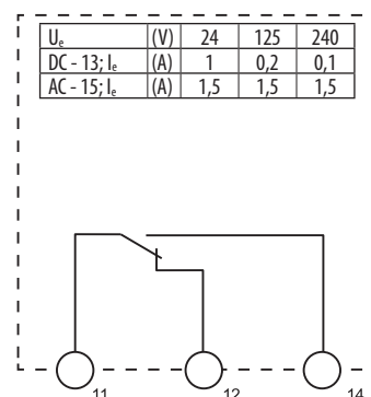
3NP1933-1GB20
